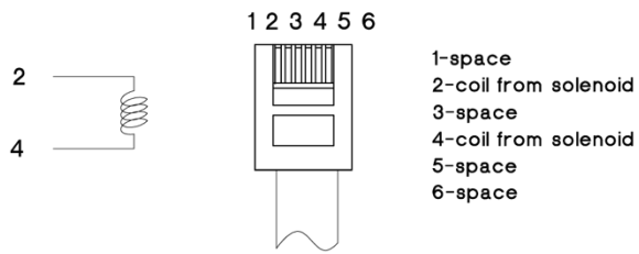
Cash box output interface
